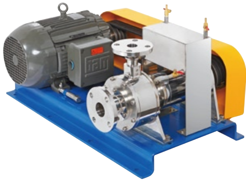
▲ 臥式皮帶傳動型 Horizontal Belt Transmission Type
